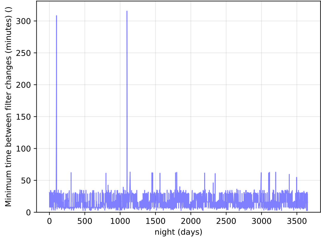
ddf_acor_sf10_Isf40_Isr10_v3.4_10yrs Per Night: Minimum time between filter changes (minutes)
