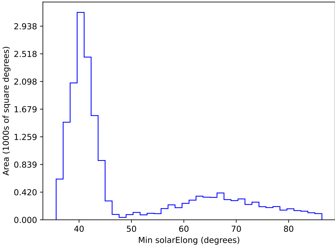
ddf_acor_sf10_lsf40_lsr10_v3.4_10yrs WFD z band: Min solarElong
