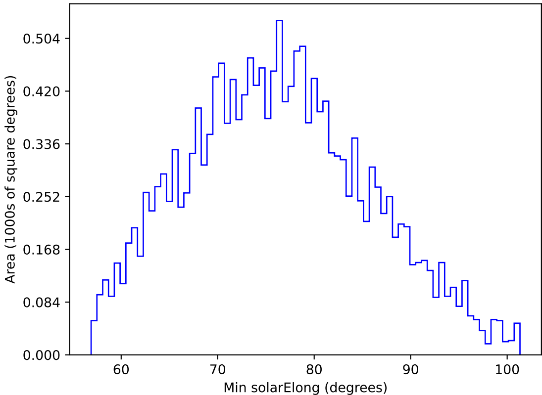
ddf_acor_sf10_lsf40_lsr10_v3.4_10yrs WFD u band: Min solarElong
