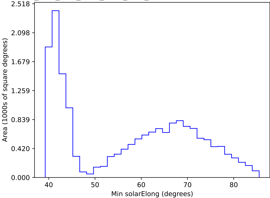
ddf_acor_sf10_lsf40_lsr10_v3.4_10yrs WFD r band: Min solarElong
