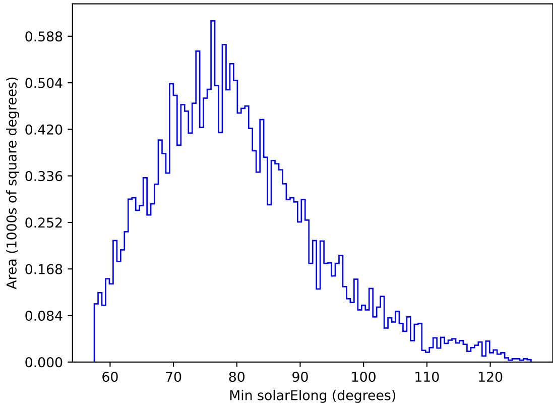
ddf_acor_sf10_lsf40_lsr10_v3.4_10yrs All sky u band: Min solarElong
