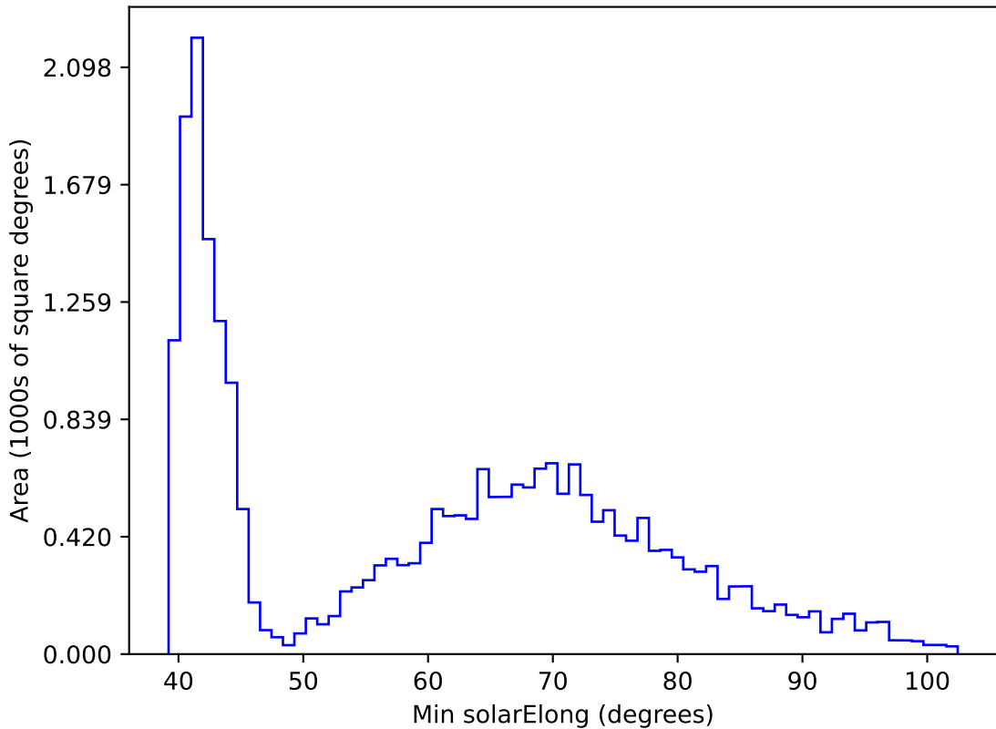
ddf_acor_sf10_ls40_lsr10_v3.4_10yrs All sky r band: Min solarElong
