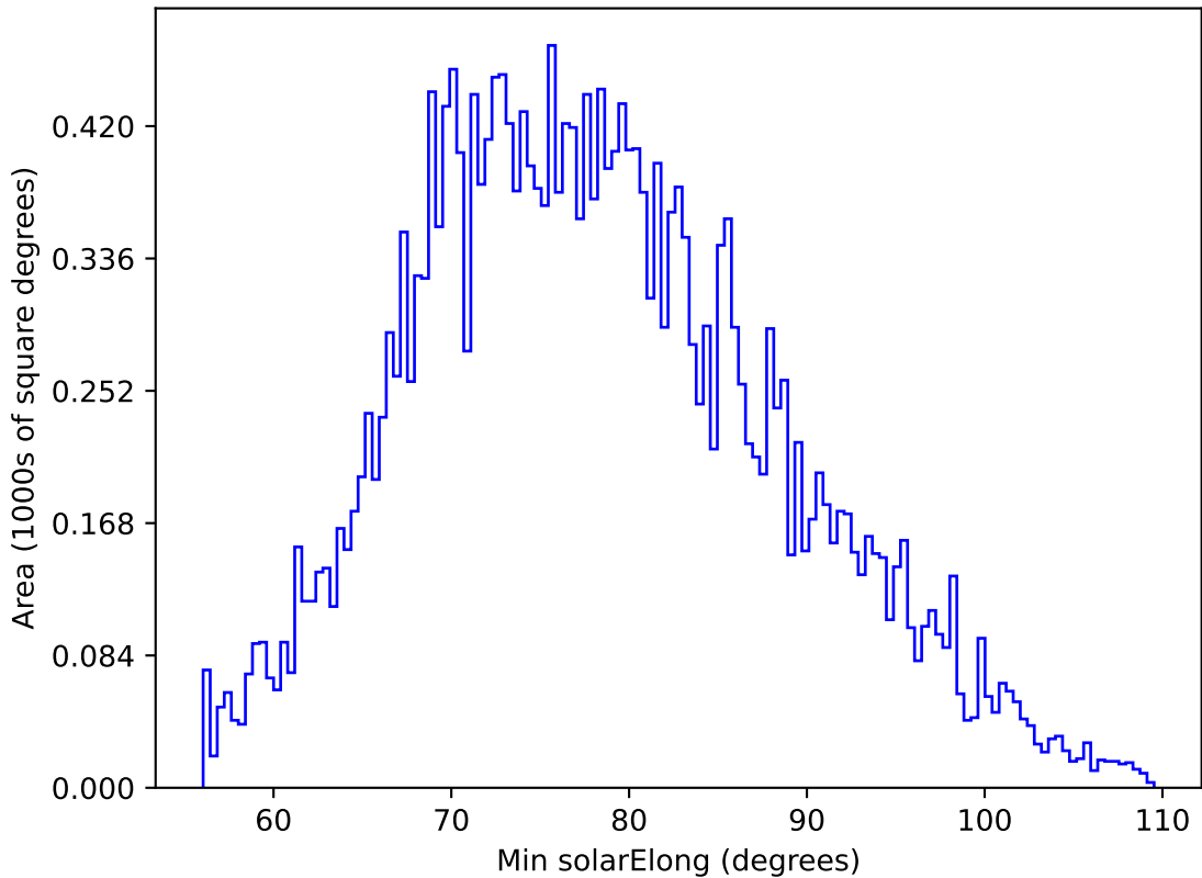
ddf_acor_sf10_lsf40_lsr10_v3.4_10yrs All sky g band: Min solarElong
