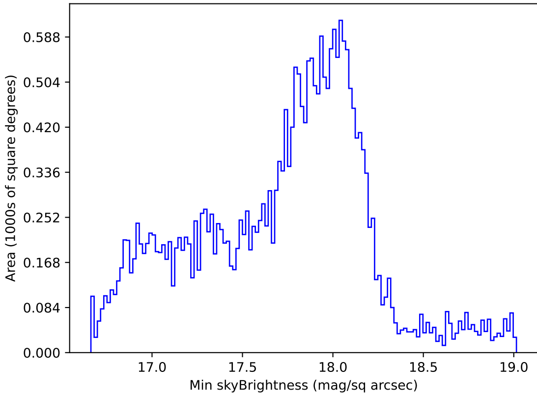
ddf_acor_sf10_lsf40_lsr10_v3.4_10yrs Yr 1 all bands: Min skyBrightness
