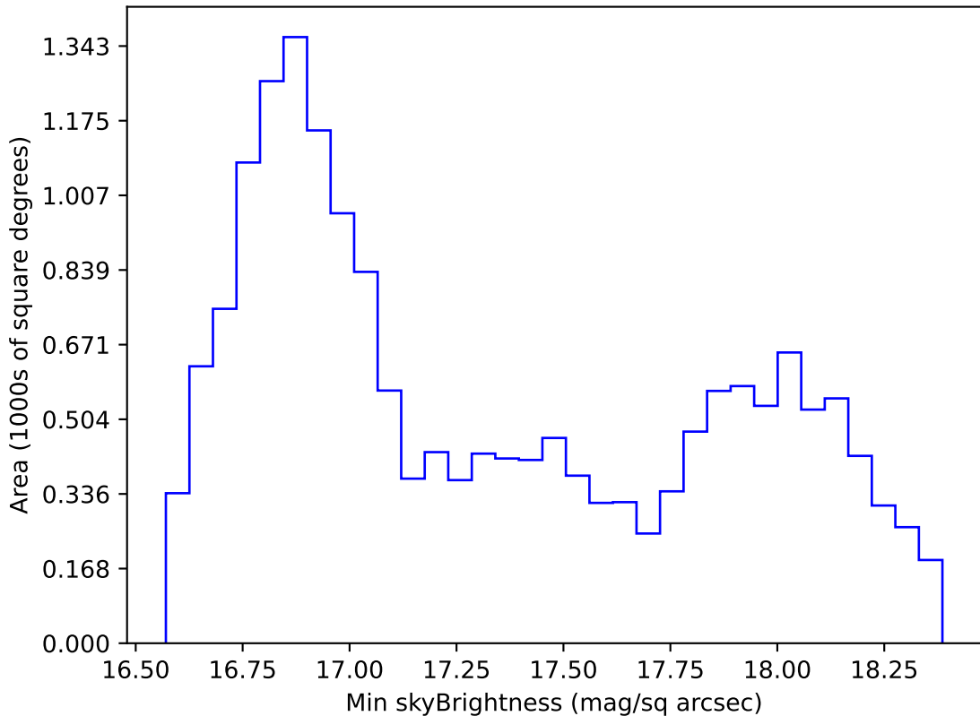
ddf_acor_sf10_lsf40_lsr10_v3.4_10yrs WFD z band: Min skyBrightness
