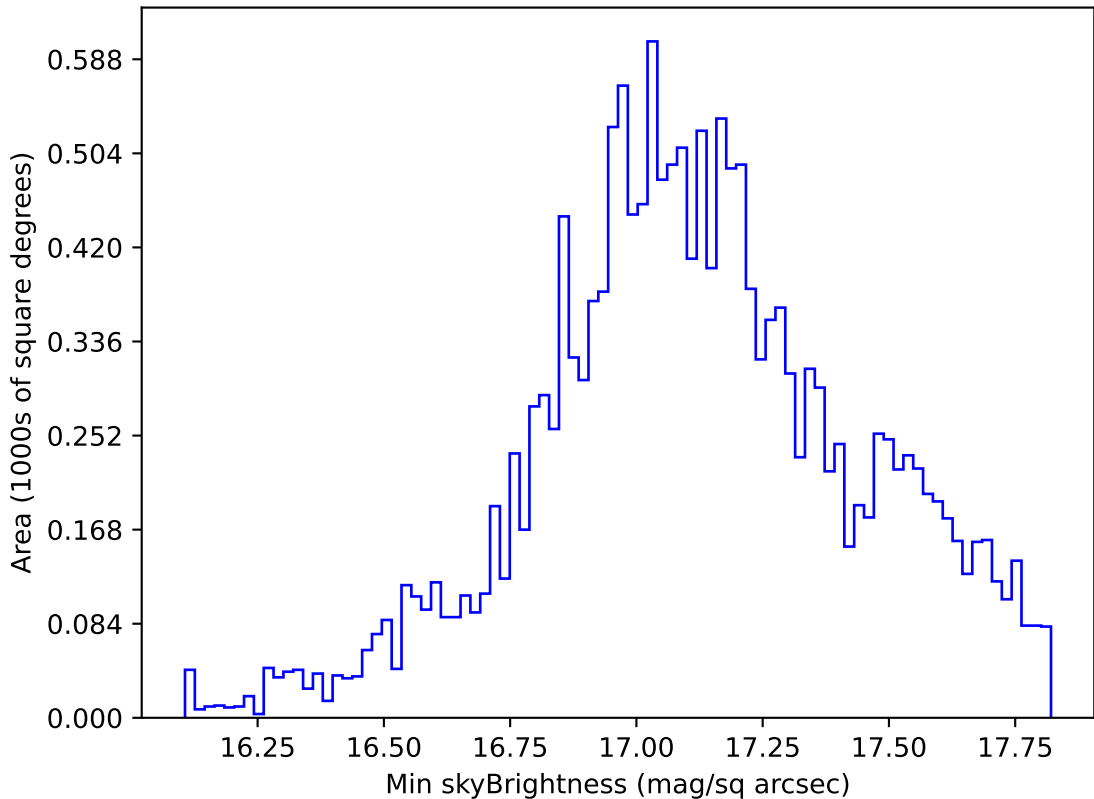
ddf_acor_sf10_lsf40_lsr10_v3.4_10yrs WFD y band: Min skyBrightness
