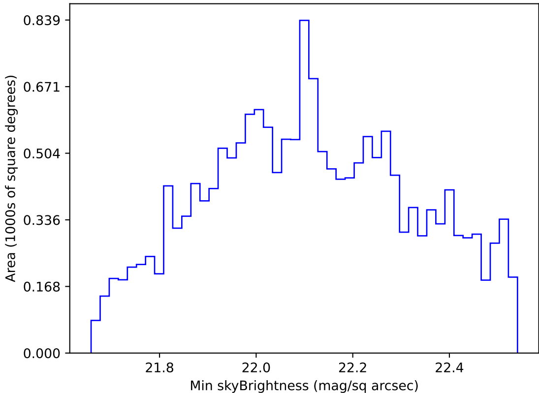
ddf_acor_sf10_lsf40_lsr10_v3.4_10yrs WFD u band: Min skyBrightness
