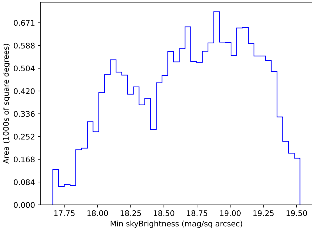
ddf_acor_sf10_lsf40_lsr10_v3.4_10yrs WFD r band: Min skyBrightness
