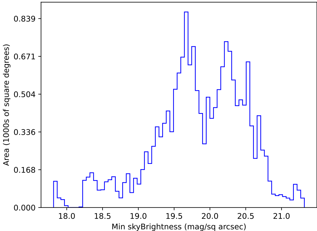
ddf_acor_sf10_lsf40_lsr10_v3.4_10yrs WFD g band: Min skyBrightness
