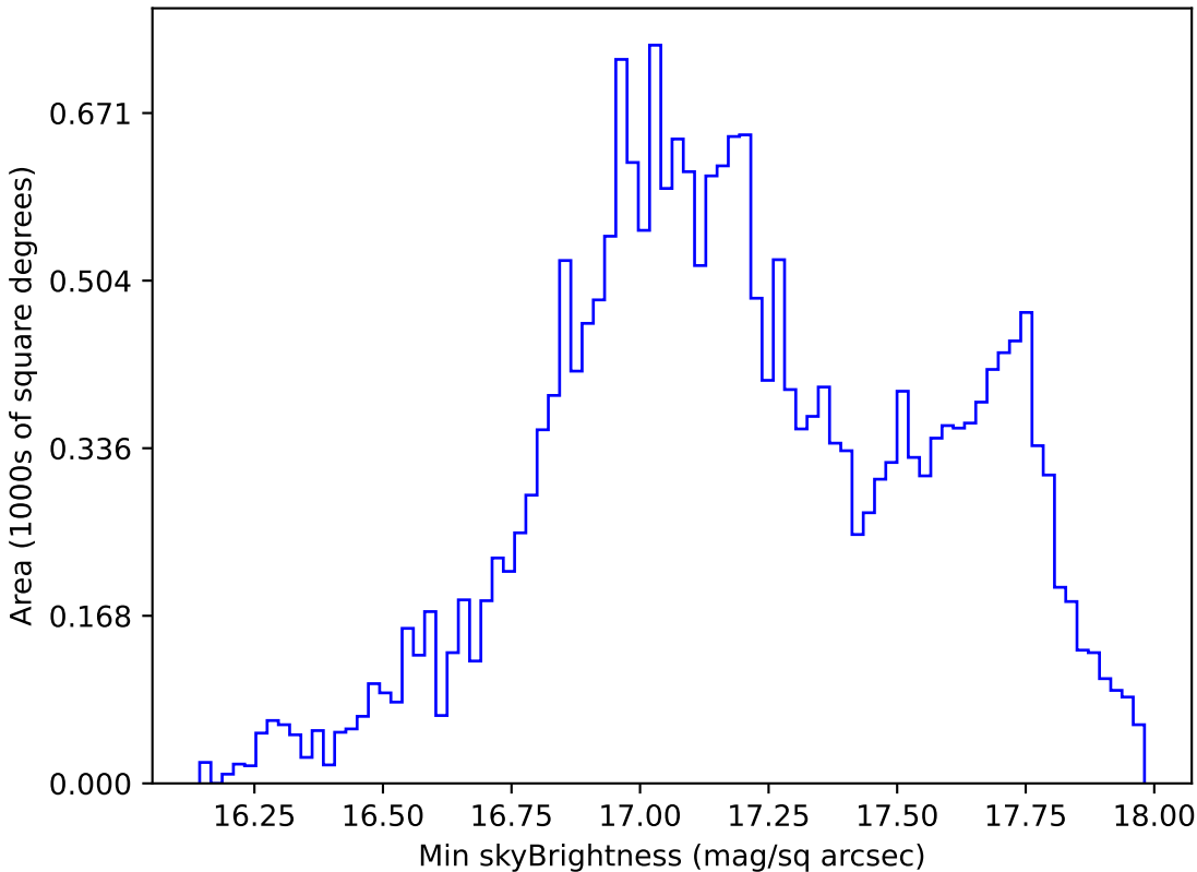
ddf_acor_sf10_lsf40_lsr10_v3.4_10yrs All sky y band: Min skyBrightness
