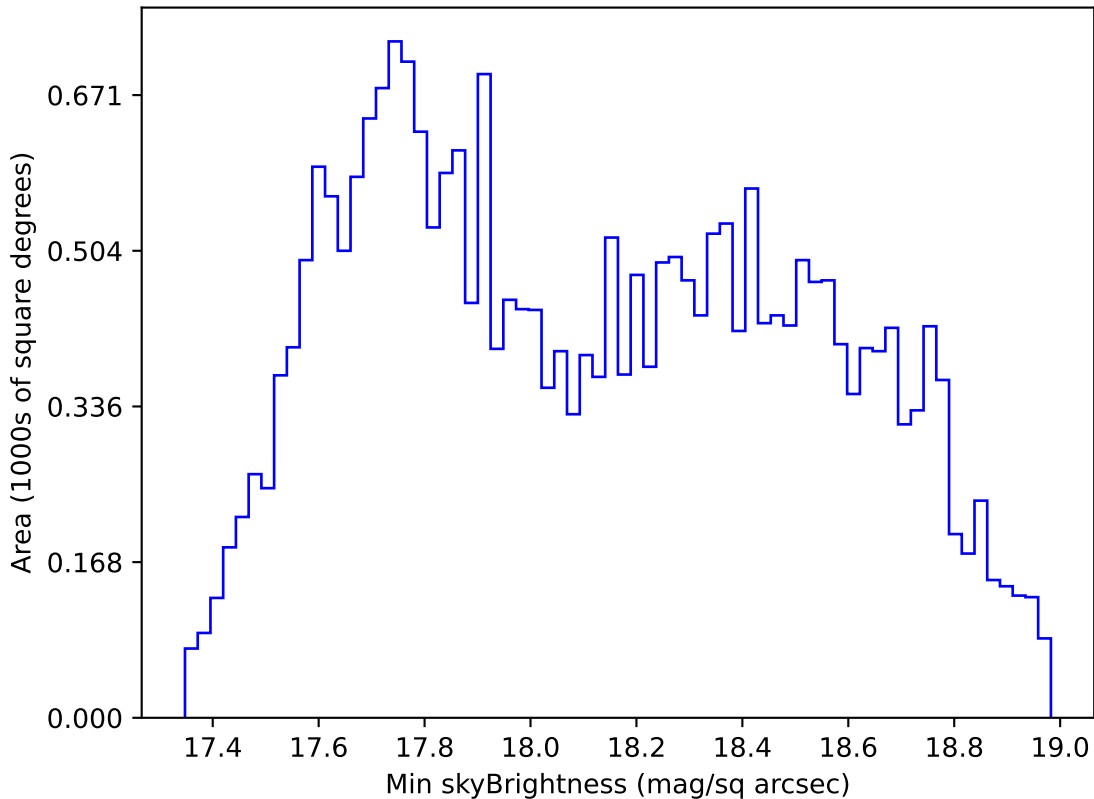
ddf_acor_sf10_lsf40_lsr10_v3.4_10yrs All sky i band: Min skyBrightness
