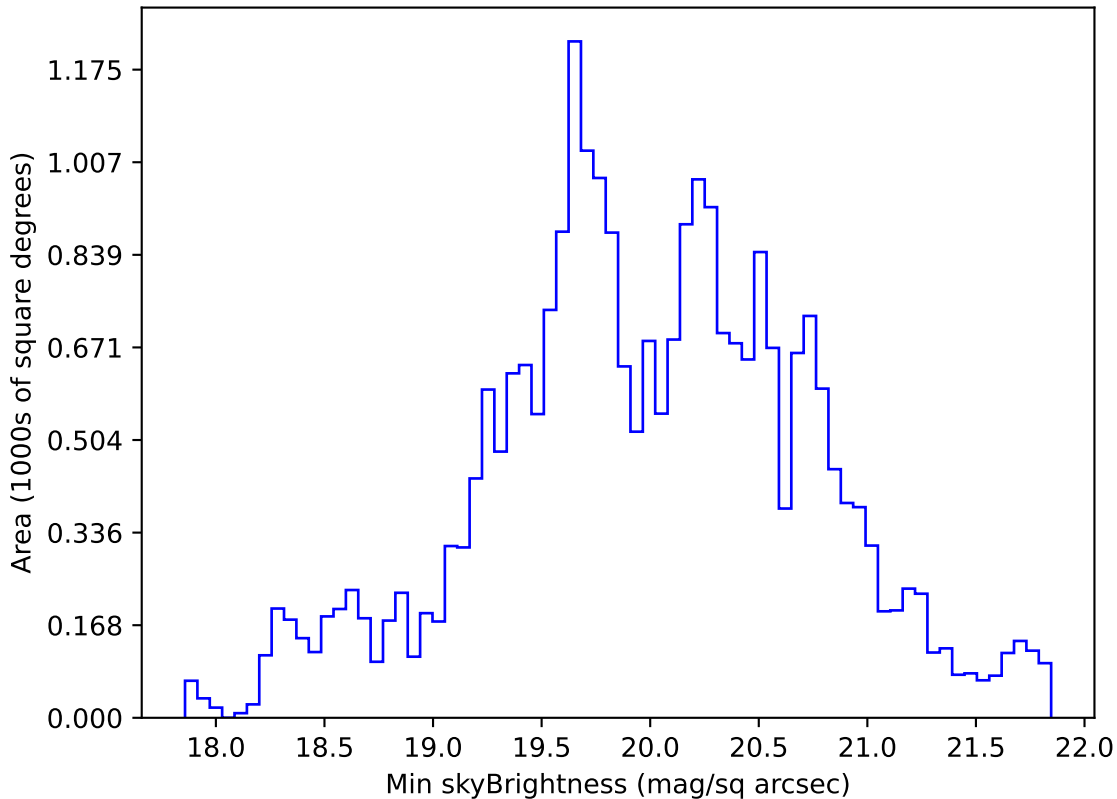
ddf_acor_sf10_lsf40_lsr10_v3.4_10yrs All sky g band: Min skyBrightness
