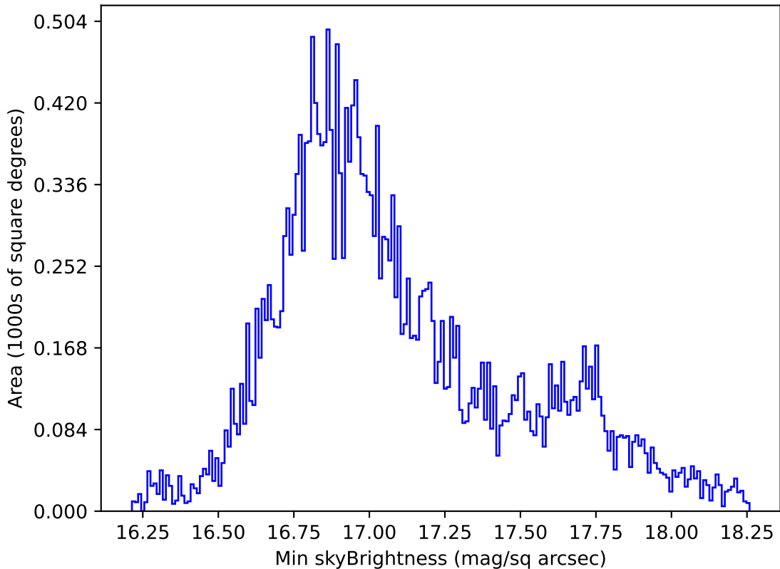
ddf_acor_sf10_lsf40_lsr10_v3.4_10yrs All sky all bands: Min skyBrightness
