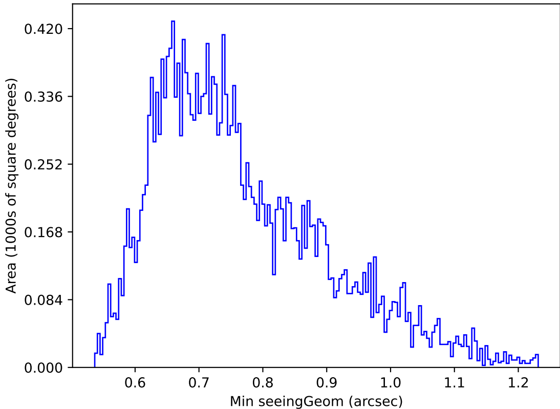
ddf_acor_sf10_ls40_lsr10_v3.4_10yrs Yr 1 u band: Min seeingGeom
