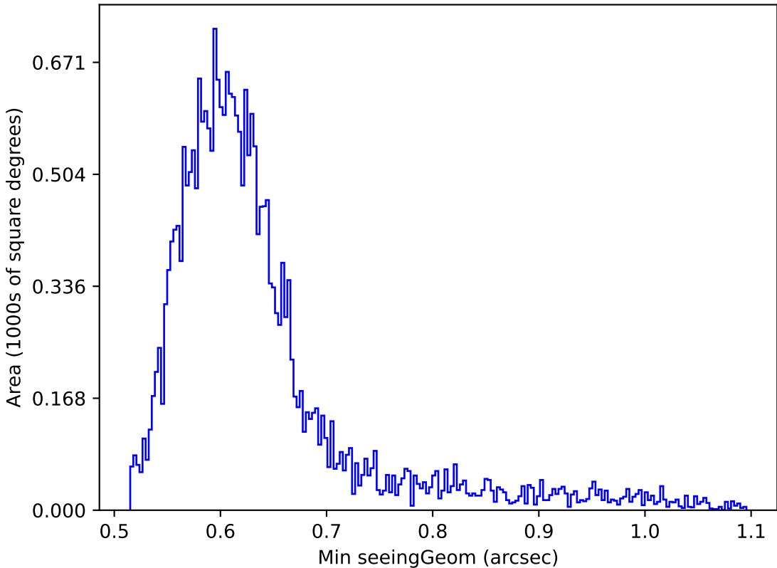
ddf_acor_sf10_lsf40_lsr10_v3.4_10yrs Yr 1 r band: Min seeingGeom
