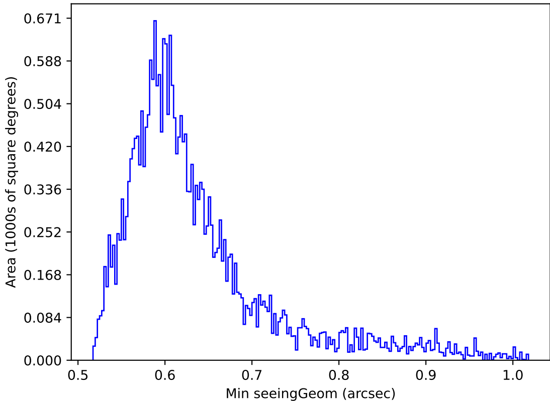
ddf_acor_sf10_lsf40_lsr10_v3.4_10yrs Yr 1 i band: Min seeingGeom
