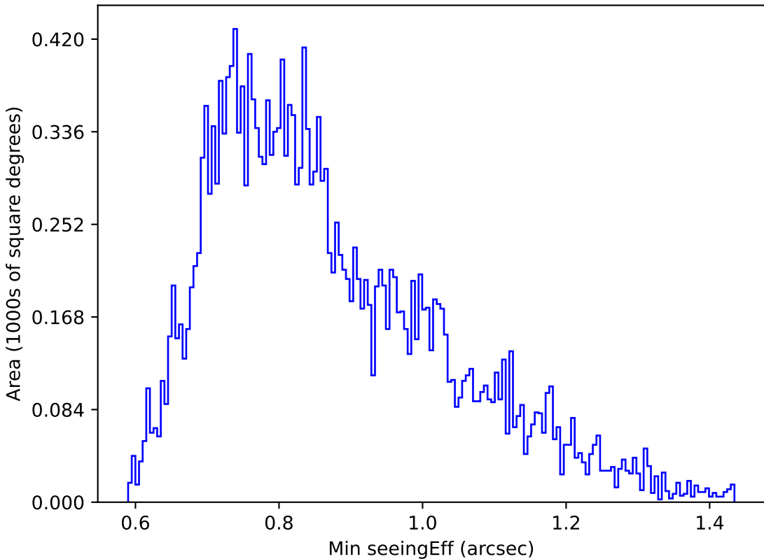
ddf_acor_sf10_lsf40_lsr10_v3.4_10yrs Yr 1 u band: Min seeingEff
