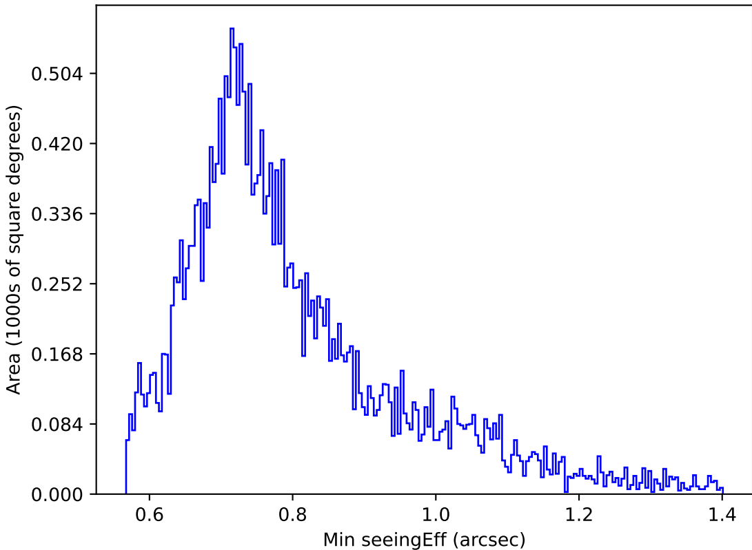
ddf_acor_sf10_lsf40_lsr10_v3.4_10yrs Yr 1 g band: Min seeingEff
