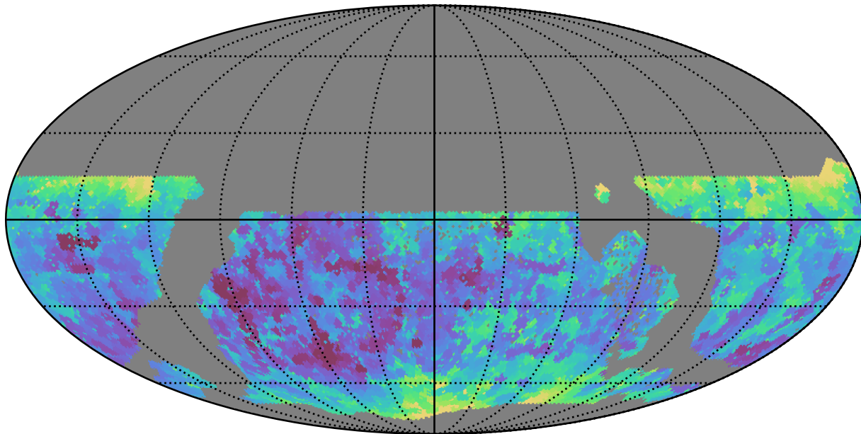
ddf_acor_sf10_lsf40_lsr10_v3.4_10yrs WFD y band: Min seeingEff
