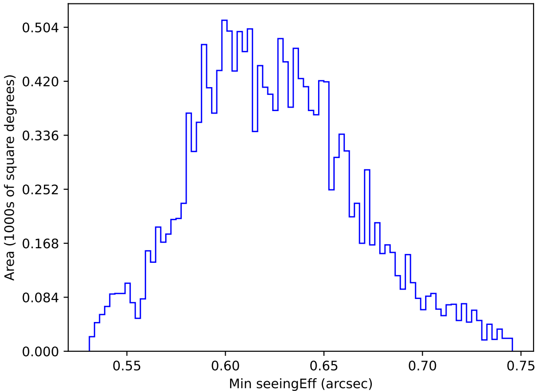
ddf_acor_sf10_lsf40_lsr10_v3.4_10yrs WFD y band: Min seeingEff
