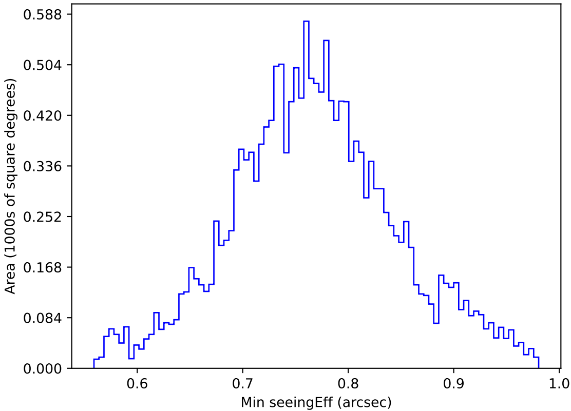
ddf_acor_sf10_lsf40_lsr10_v3.4_10yrs WFD u band: Min seeingEff
