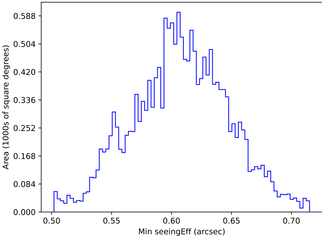
ddf_acor_sf10_lsf40_lsr10_v3.4_10yrs WFD i band: Min seeingEff
