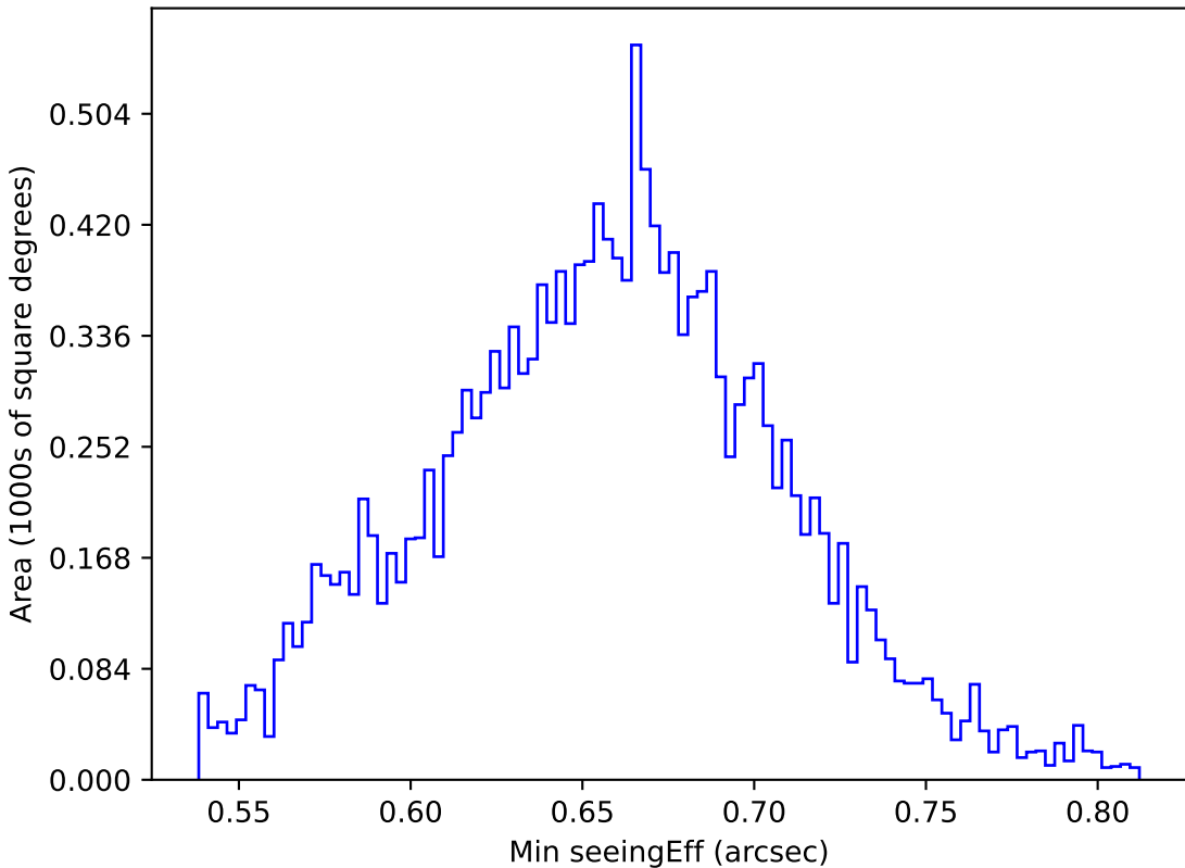
ddf_acor_sf10_lsf40_lsr10_v3.4_10yrs WFD g band: Min seeingEff
