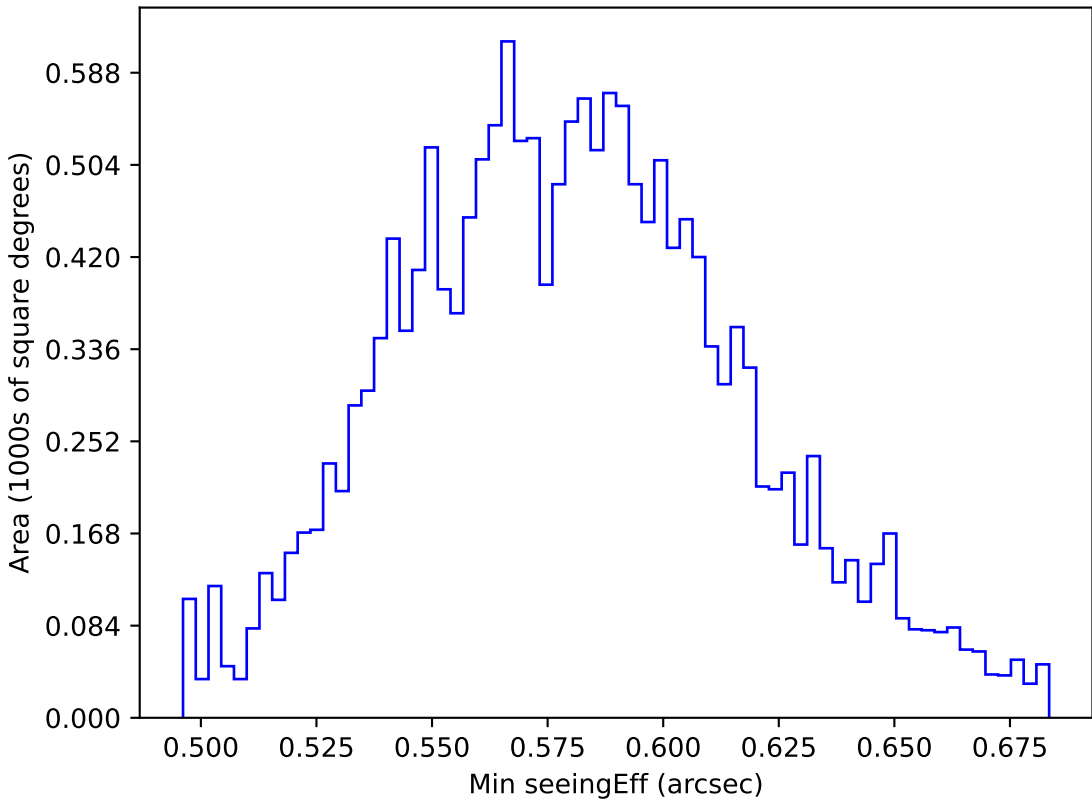
ddf_acor_sf10_lsf40_lsr10_v3.4_10yrs WFD all bands: Min seeingEff
