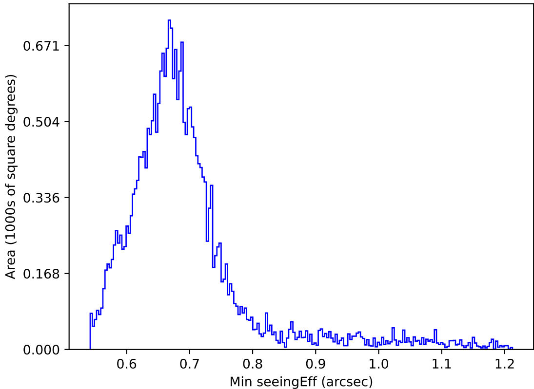
ddf_acor_sf10_lsf40_lsr10_v3.4_10yrs All sky g band: Min seeingEff
