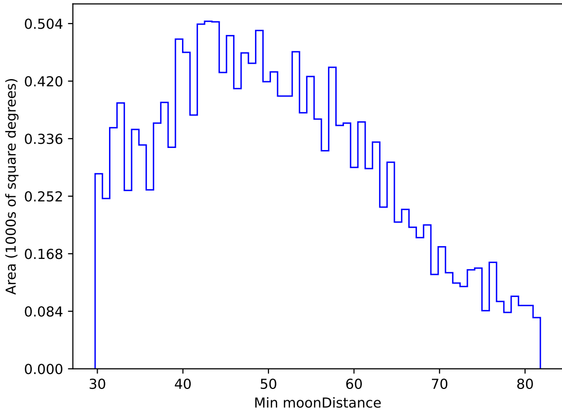
ddf_acor_sf10_lsf40_lsr10_v3.4_10yrs WFD u band: Min moonDistance
