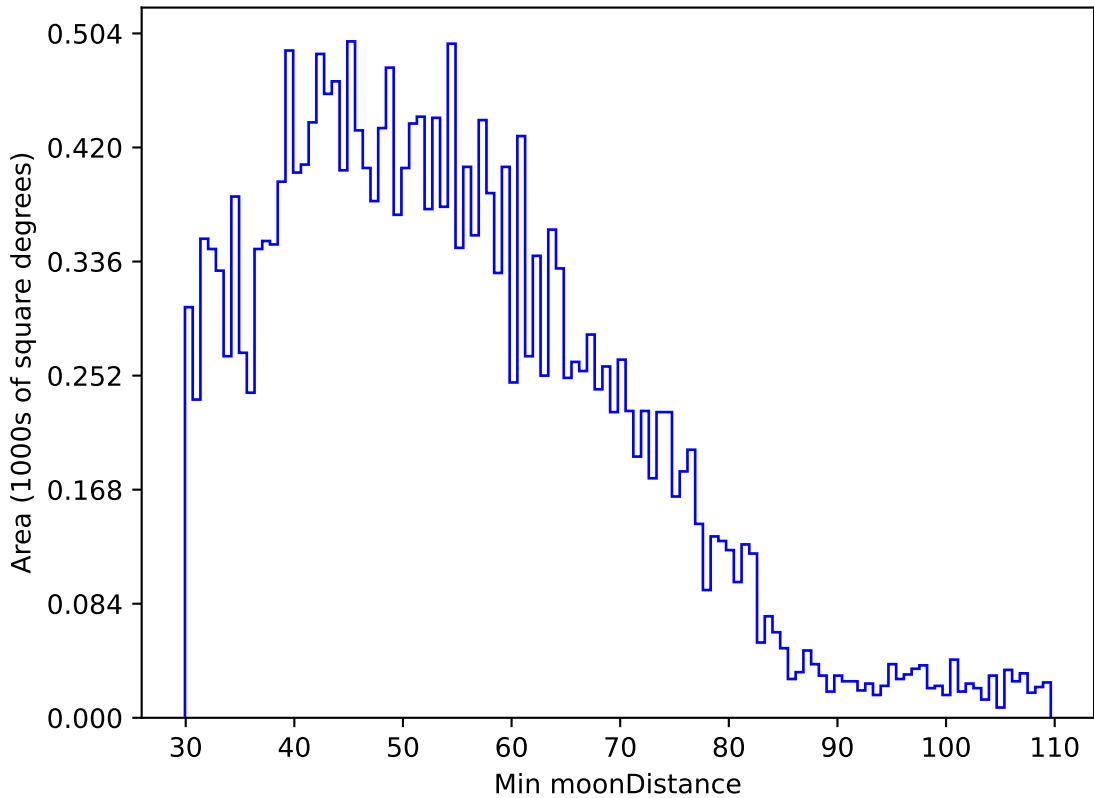
ddf_acor_sf10_lsf40_lsr10_v3.4_10yrs All sky u band: Min moonDistance
