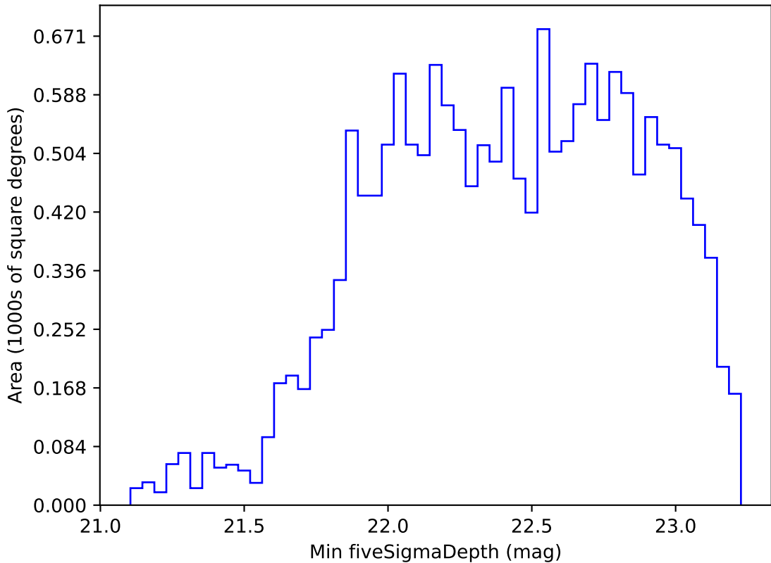
ddf_acor_sf10_lsf40_lsr10_v3.4_10yrs WFD r band: Min fiveSigmaDepth
