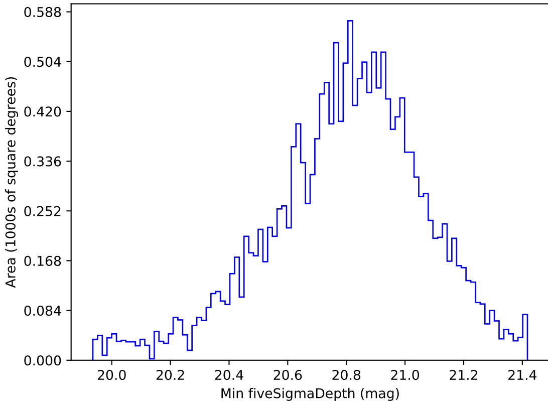
ddf_acor_sf10_lsf40_lsr10_v3.4_10yrs WFD all bands: Min fiveSigmaDepth
