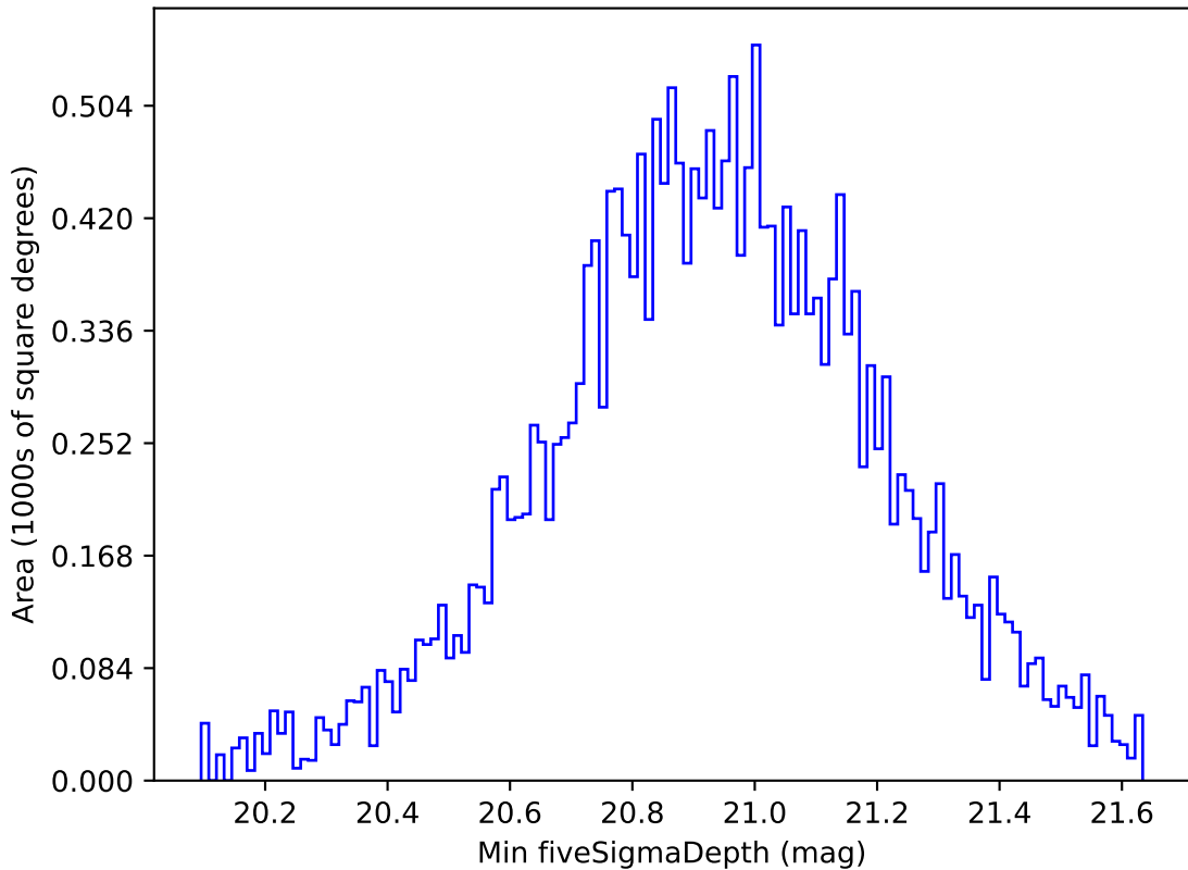
ddf_acor_sf10_lsf40_lsr10_v3.4_10yrs All sky y band: Min fiveSigmaDepth
