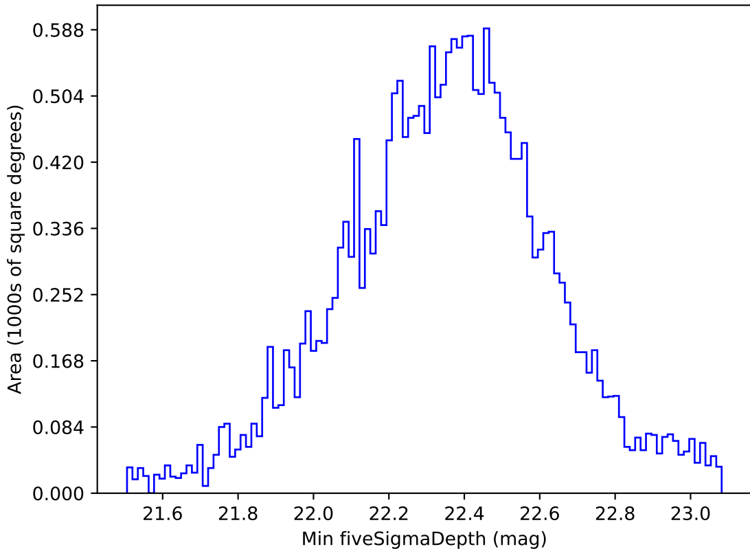
ddf_acor_sf10_lsf40_lsr10_v3.4_10yrs All sky u band: Min fiveSigmaDepth
