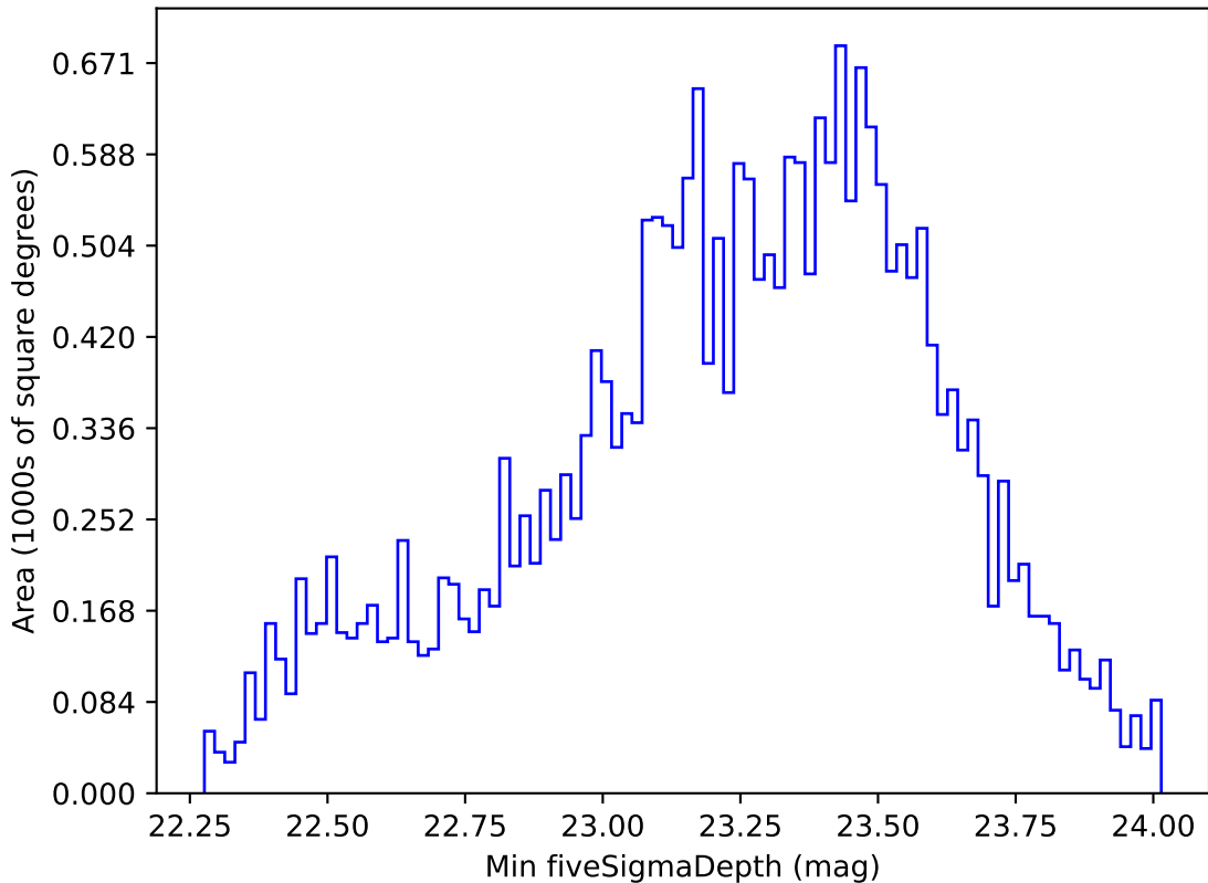
ddf_acor_sf10_lsf40_lsr10_v3.4_10yrs All sky g band: Min fiveSigmaDepth
