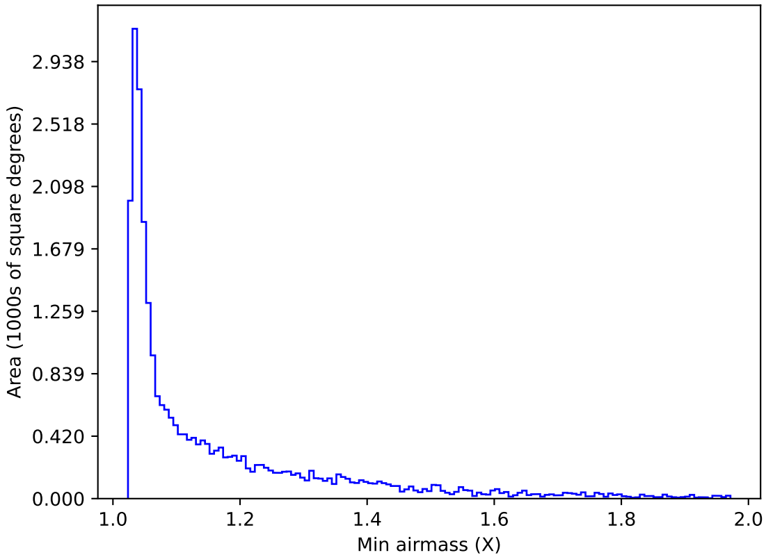
ddf_acor_sf10_lsf40_lsr10_v3.4_10yrs Yr 1 r band: Min airmass
