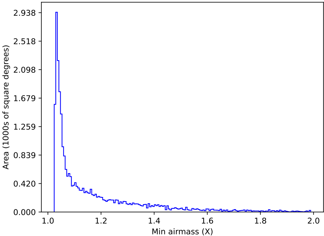
ddf_acor_sf10_lsf40_lsr10_v3.4_10yrs Yr 1 i band: Min airmass
