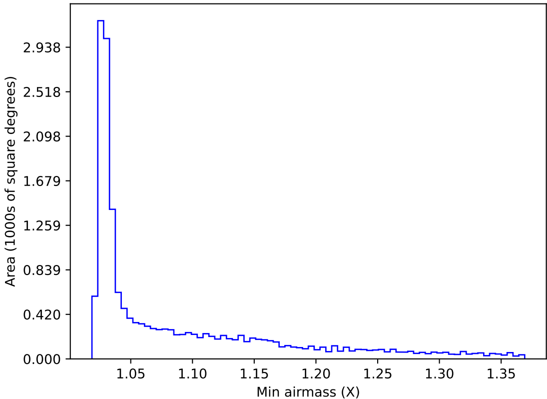
ddf_acor_sf10_lsf40_lsr10_v3.4_10yrs WFD z band: Min airmass
