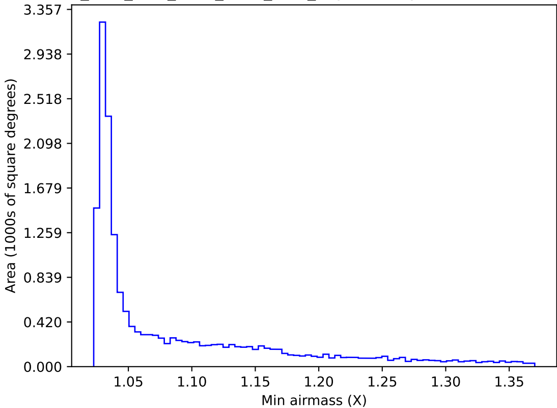
ddf_acor_sf10_lsf40_lsr10_v3.4_10yrs WFD y band: Min airmass
