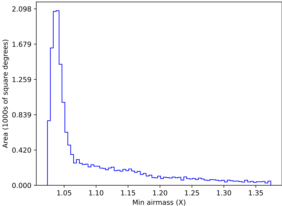
ddf_acor_sf10_lsf40_lsr10_v3.4_10yrs WFD u band: Min airmass
