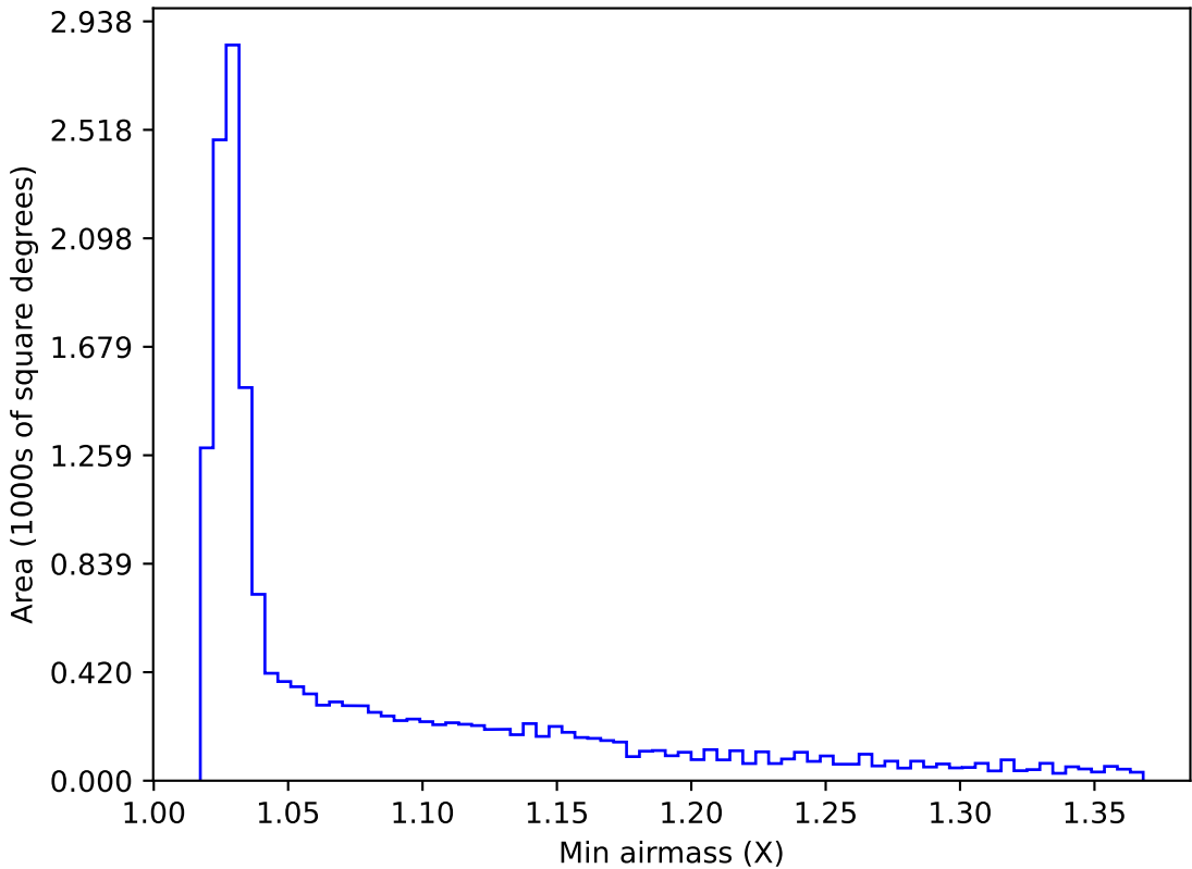
ddf_acor_sf10_lsf40_lsr10_v3.4_10yrs WFD r band: Min airmass
