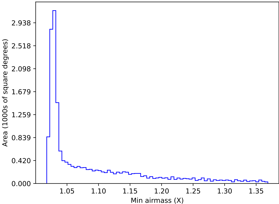
ddf_acor_sf10_lsf40_lsr10_v3.4_10yrs WFD i band: Min airmass
