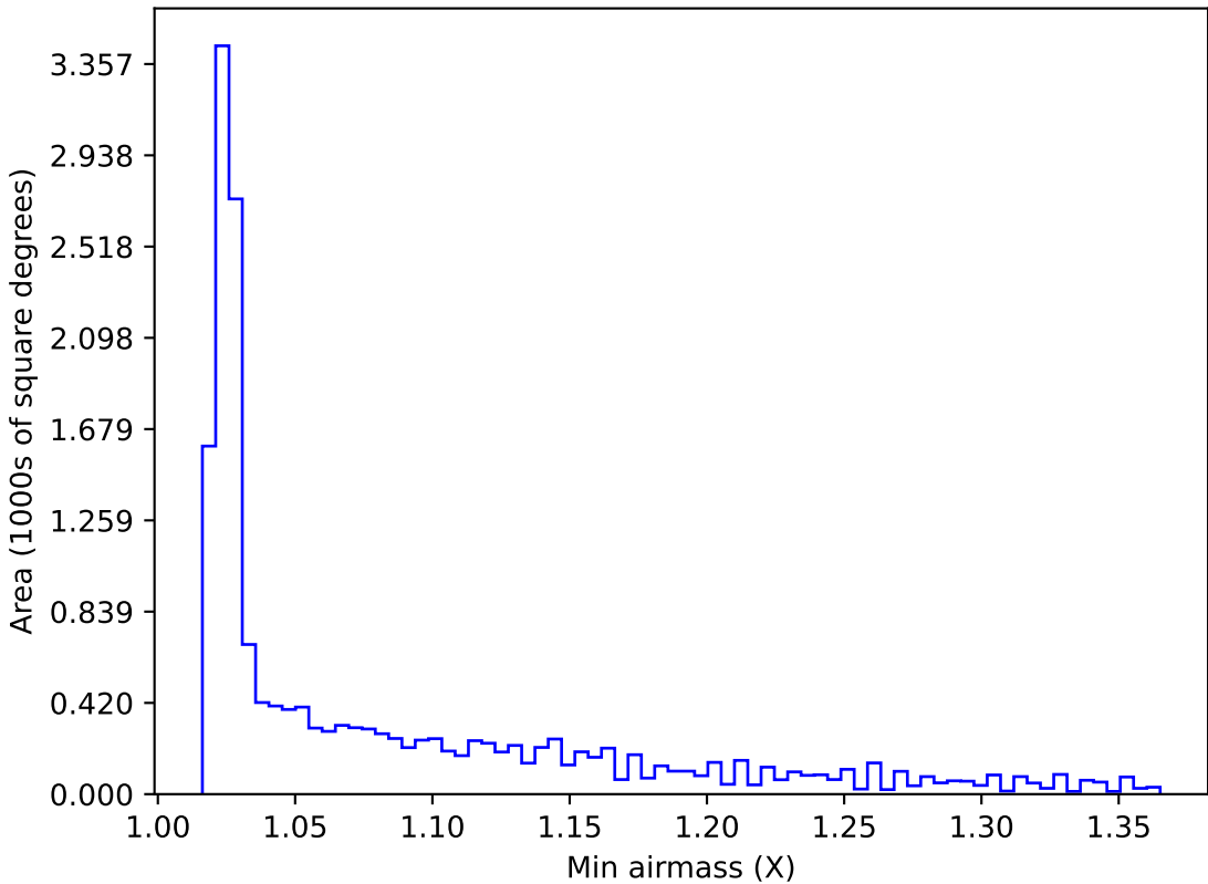
ddf_acor_sf10_lsf40_lsr10_v3.4_10yrs WFD all bands: Min airmass
