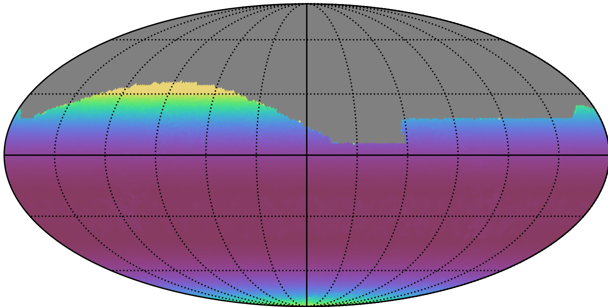
ddf_acor_sf10_lsf40_lsr10_v3.4_10yrs All sky r band: Min airmass
