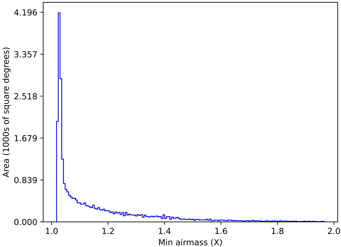
ddf_acor_sf10_lsf40_lsr10_v3.4_10yrs All sky r band: Min airmass
