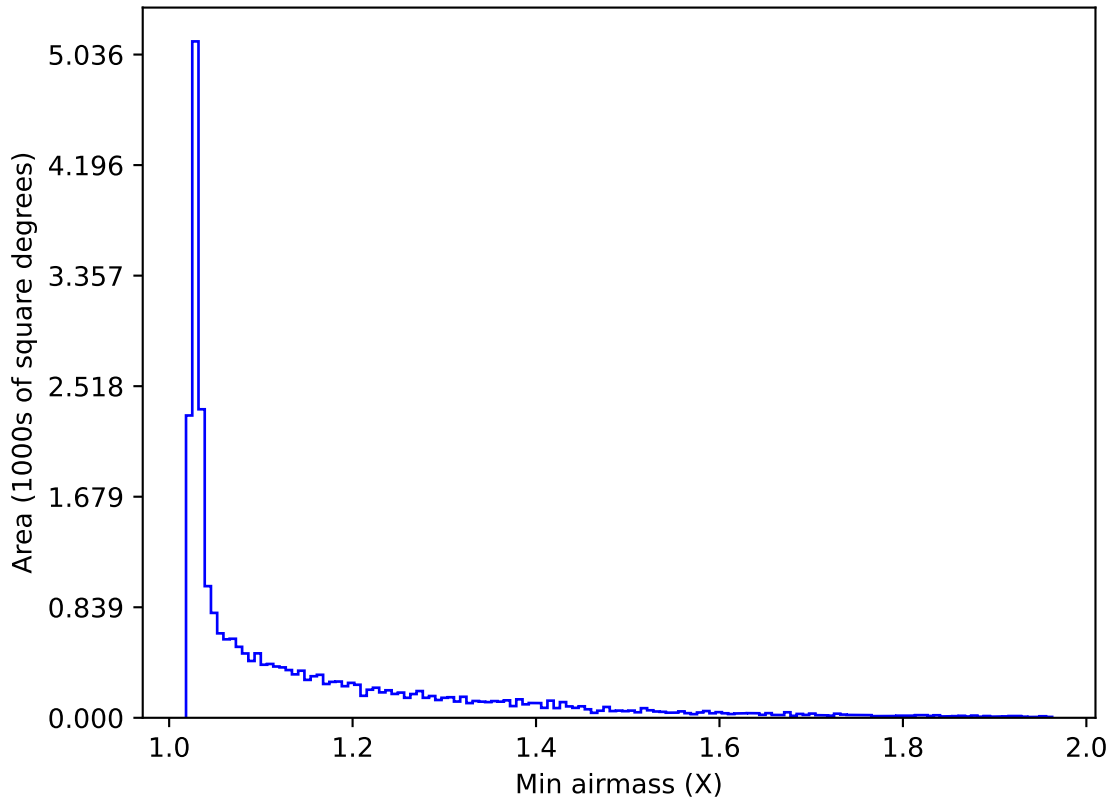
ddf_acor_sf10_lsf40_lsr10_v3.4_10yrs All sky i band: Min airmass
