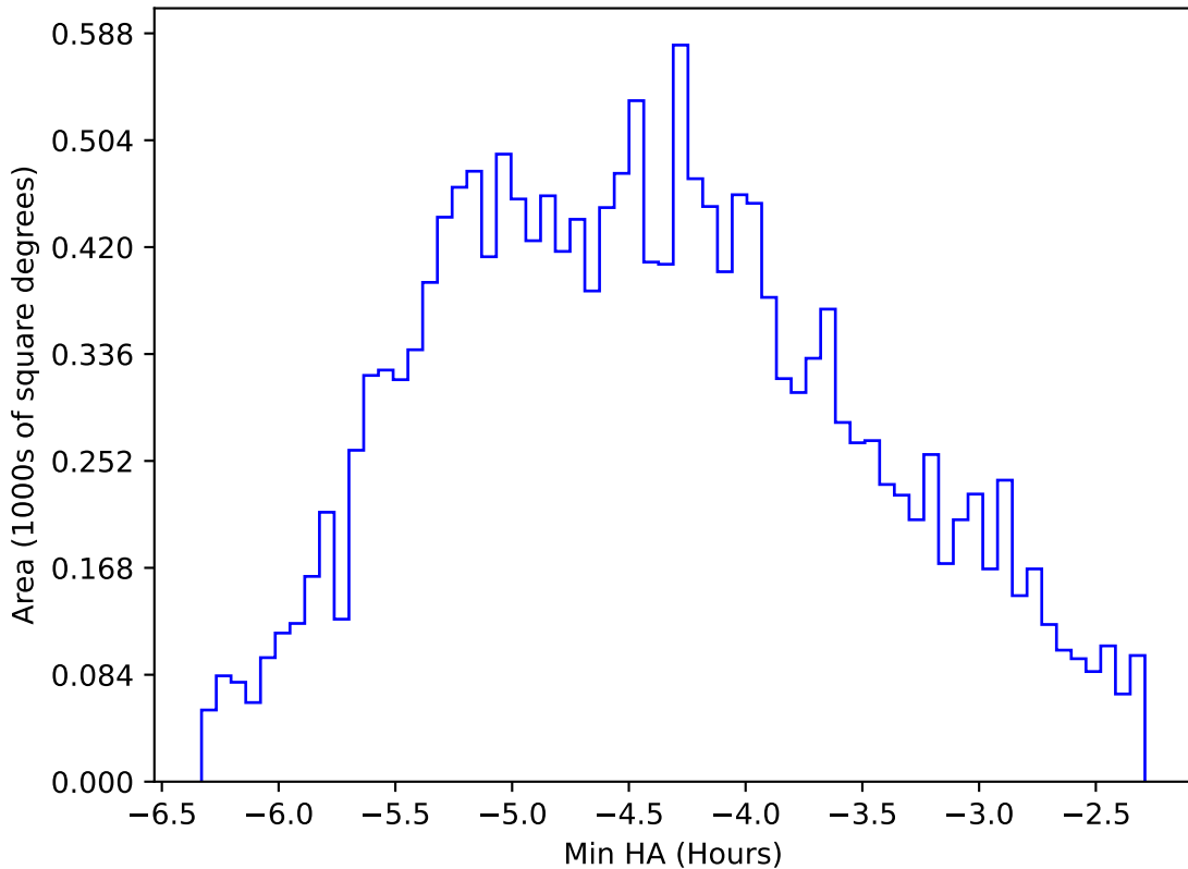
ddf_acor_sf10_lsf40_lsr10_v3.4_10yrs WFD r band: Min HA
