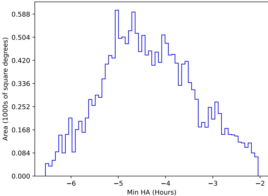
ddf_acor_sf10_ls40_lsr10_v3.4_10yrs WFD i band: Min HA
