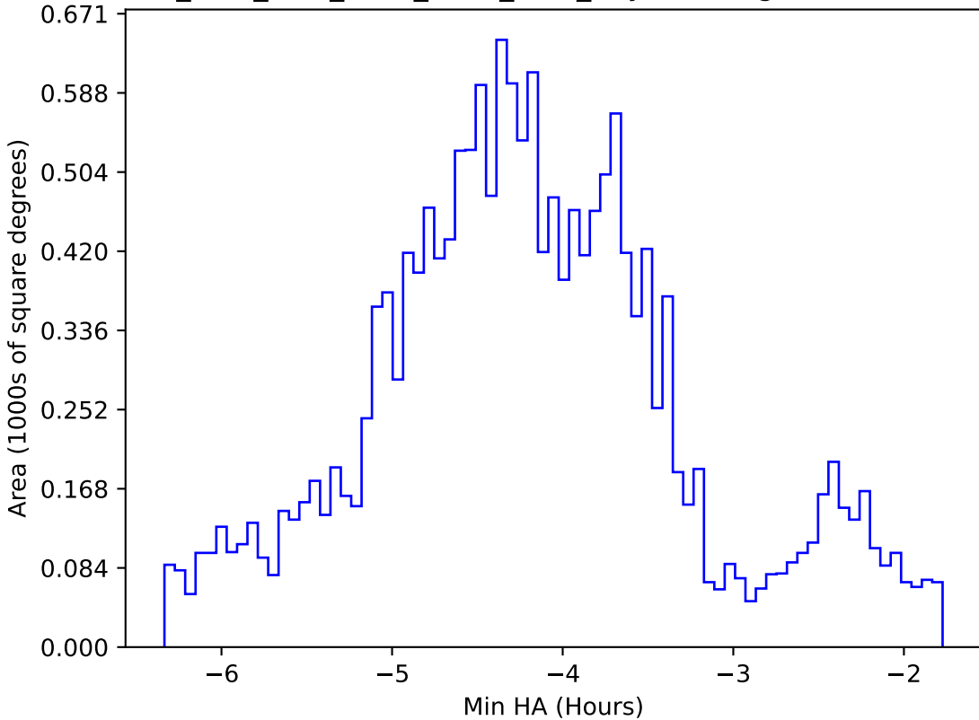
ddf_acor_sf10_lsf40_lsr10_v3.4_10yrs WFD g band: Min HA
